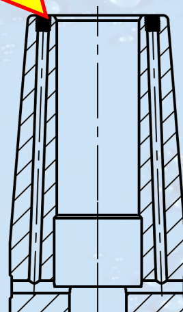
2 Pluggable Angled Coolant Ports
