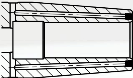
2 Pluggable Angled Coolant Ports
